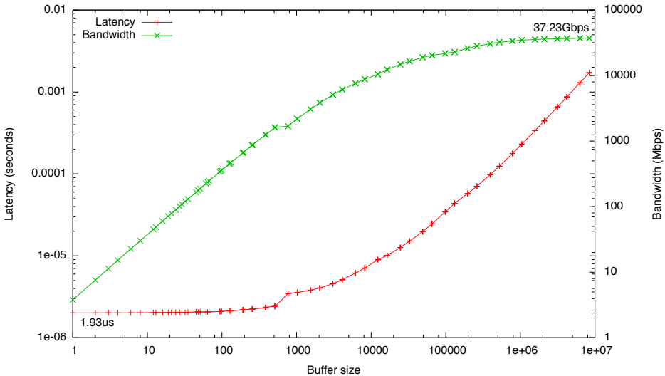
NetPIPE on Intel Xeon E5-2690 (v1) with Cisco VIC 1285 and usNIC (back-to-back; no network switch)
