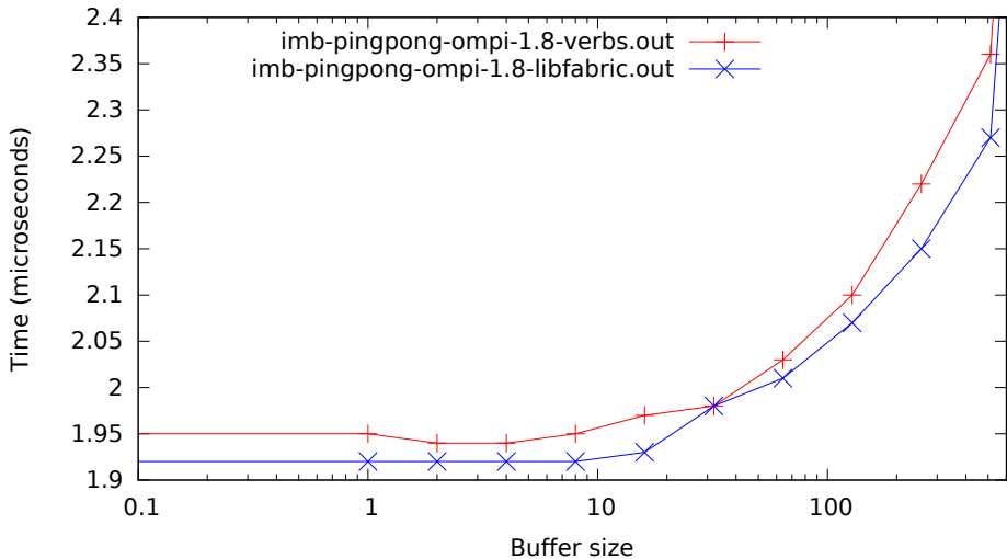
Open MPI with usNIC: IMB PingPong Latency
