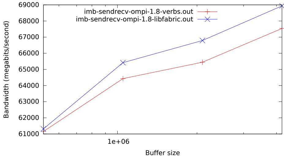
Open MPI with usNIC: IMB SendRecv Bandwidth
