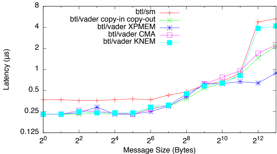
IMB Pingpong Latency (IMB Pingpong)
