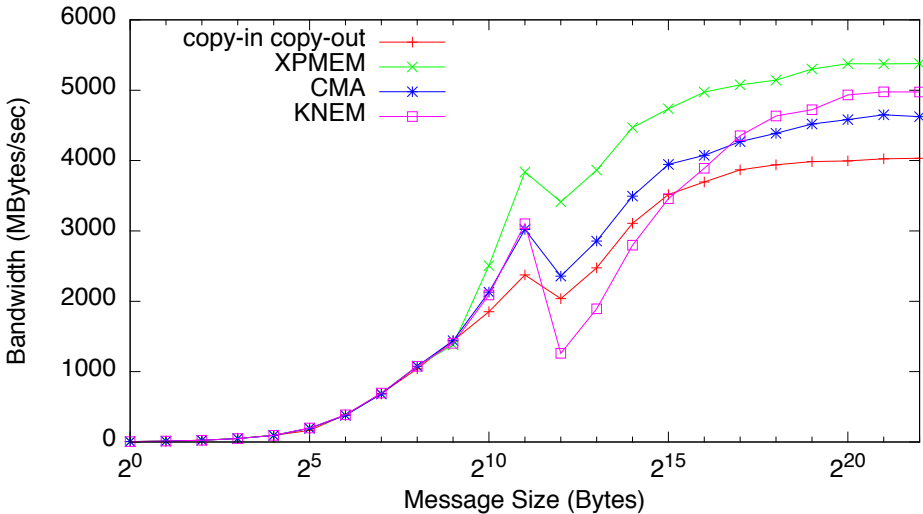
IMB Sendrecv Off-cache Bandwidth (IMB Sendrecv -off_cache -1)
